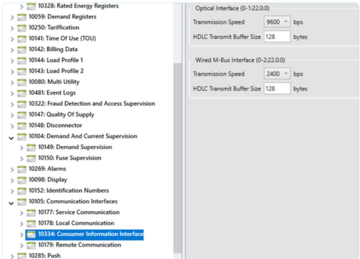
Customer Information Interface
