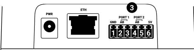
Figure 3: Communication interfaces pinout (marked as number 3)
