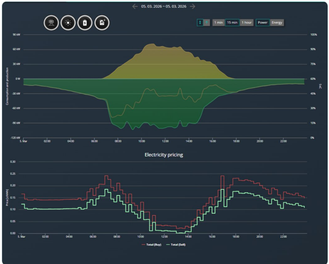
Load forecast and solar production forecast
